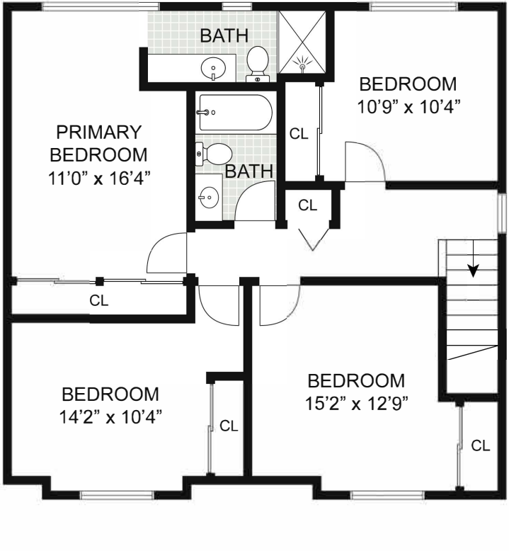
UPPER FLOOR
