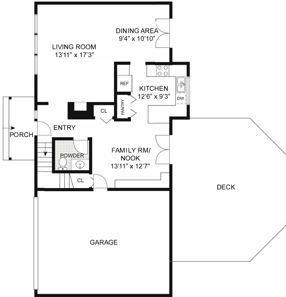
FIRST FLOOR
