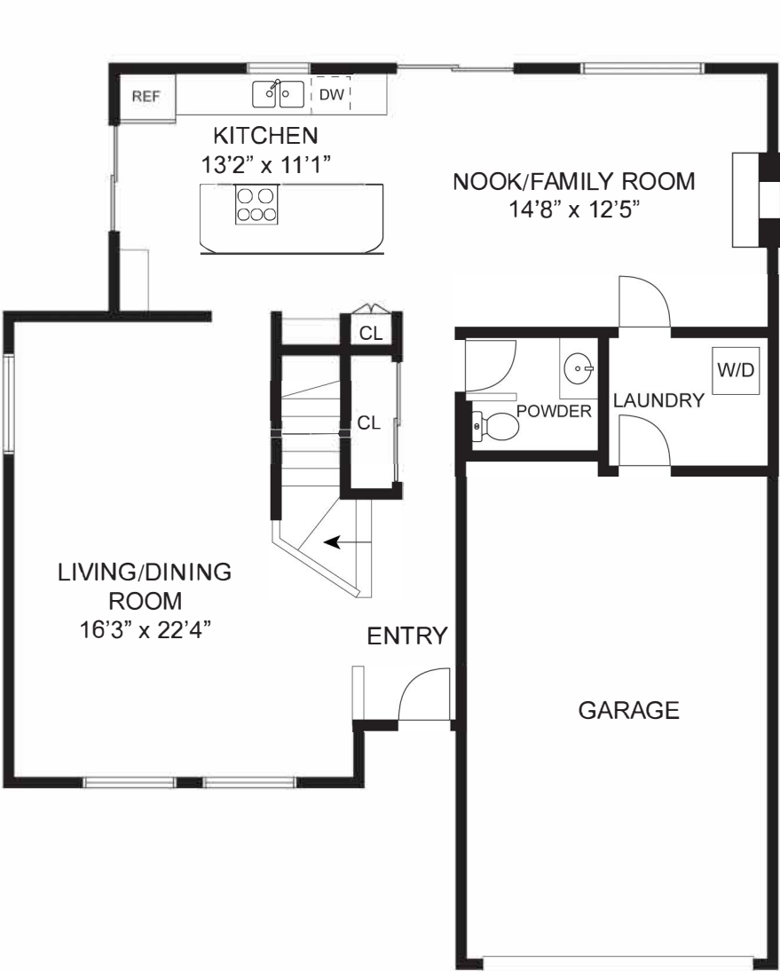
FIRST FLOOR
